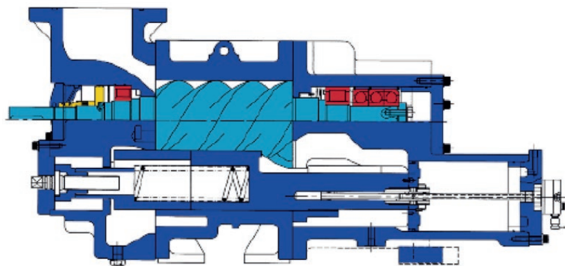
Sectional view of typical XRV screw compressor
