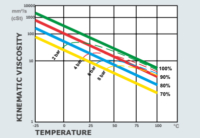
KINEMATIC VISCOSITY AND VAPOUR PRESSURE OF SUNISO® SL32 - R134a MIXTURE
