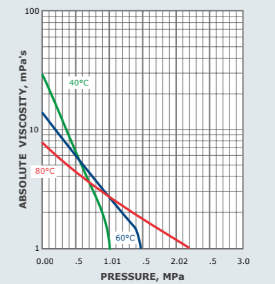
VISCOSITY - PRESSURE CHART FOR SOLUTIONS OF R-134a in SUNISO® SL32 at 40°C, 60°C, 80°C
